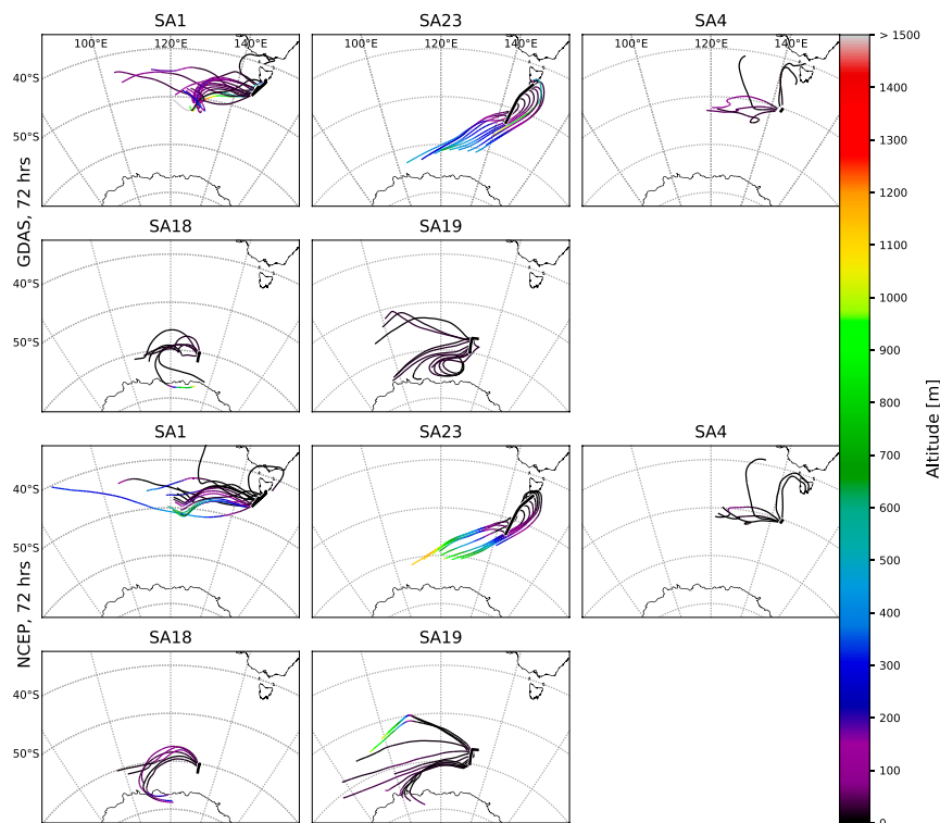
Fig. 4. Three-day back trajectories calculated using HYSPPLIT and two different meteorological datasets (GDAS 1° and NCEP/NCAR reanalysis), initiated at each sampling date and location, and 25-m altitude.
