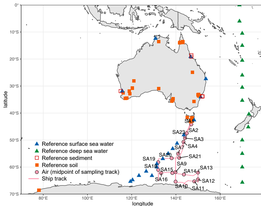
Fig. 1. Ship track, air sampling sites (SA#), and locations of collection of reference samples: Australian and Antarctic soils, ocean sediments, surface sea water, and deep sea water. Further details on samples and references are in SI Appendix, Table S1.
